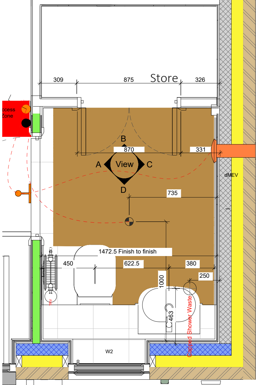
1 Ground Floor W/C Layout 1 : 20
