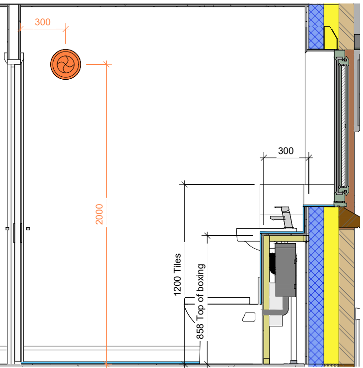
A WC - View A 1 : 25
