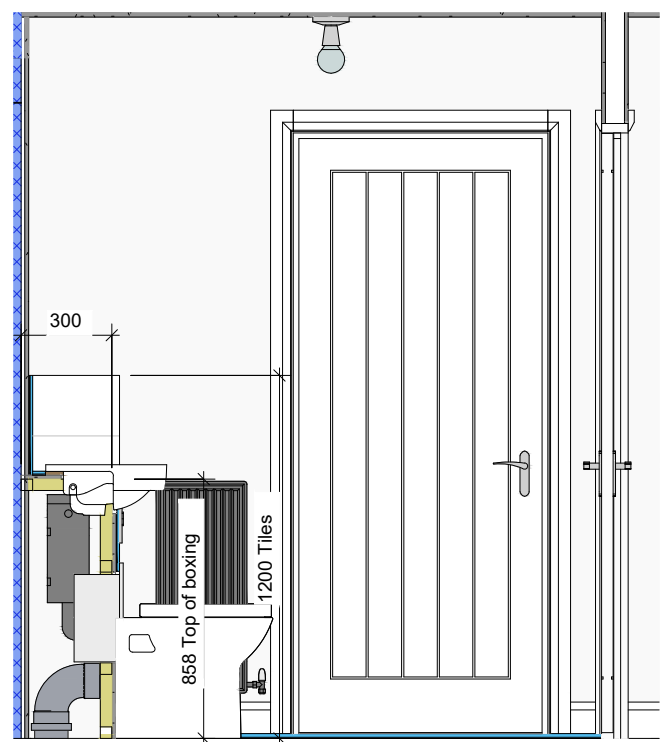
A WC - View A 1 : 25
